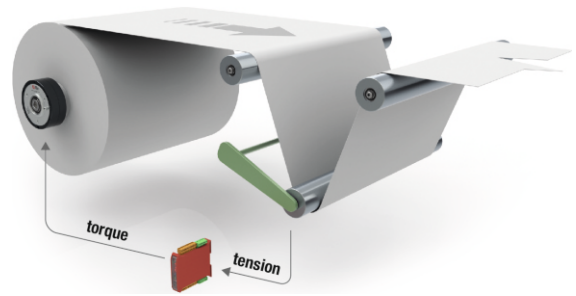
Regulation in torque with dancing roller
