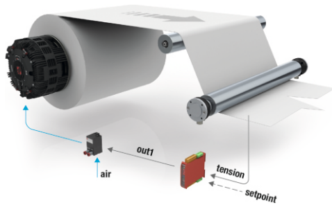
Regulation in torque with load cells
